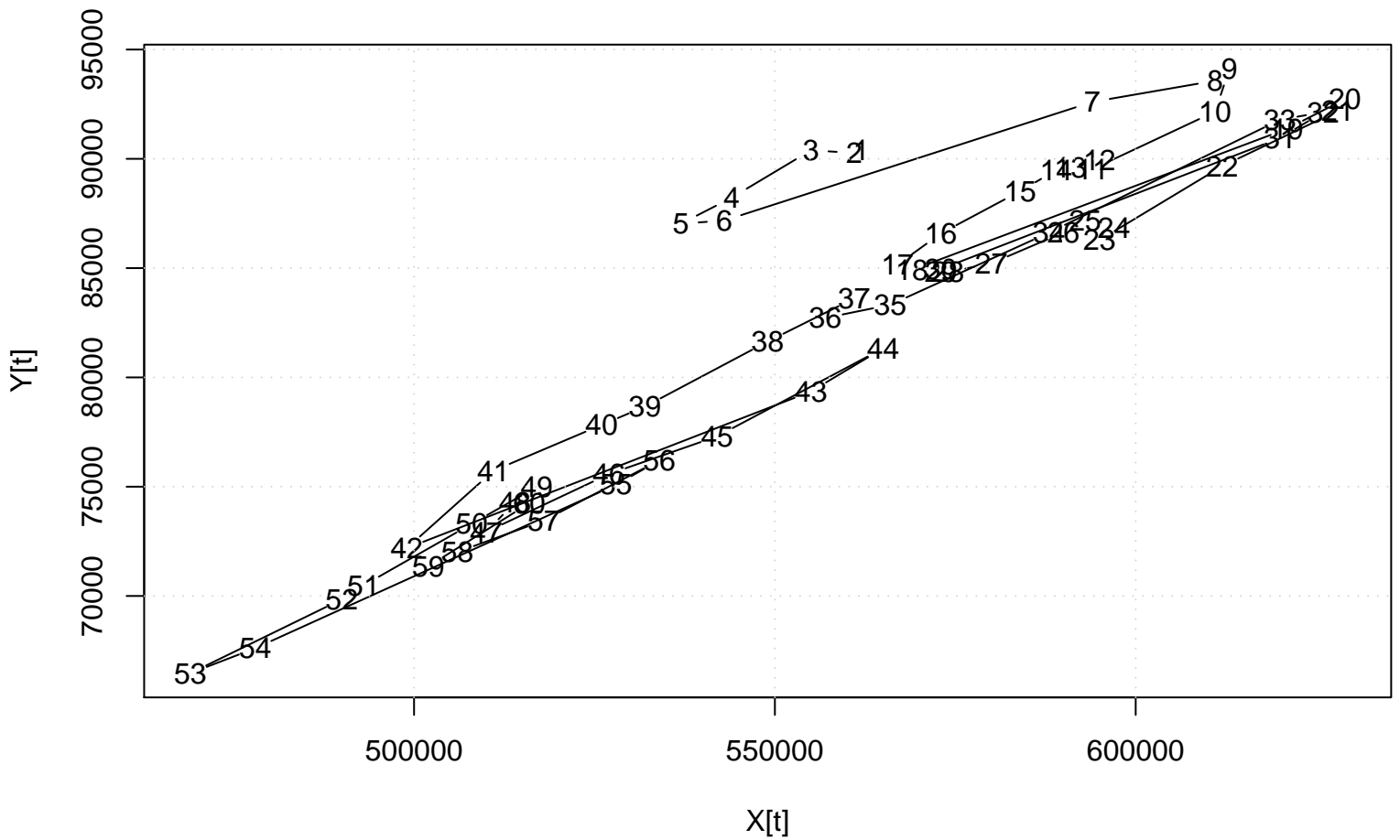
Scatter Plot
