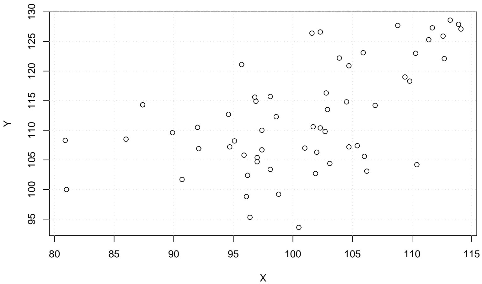
Scatterplot
