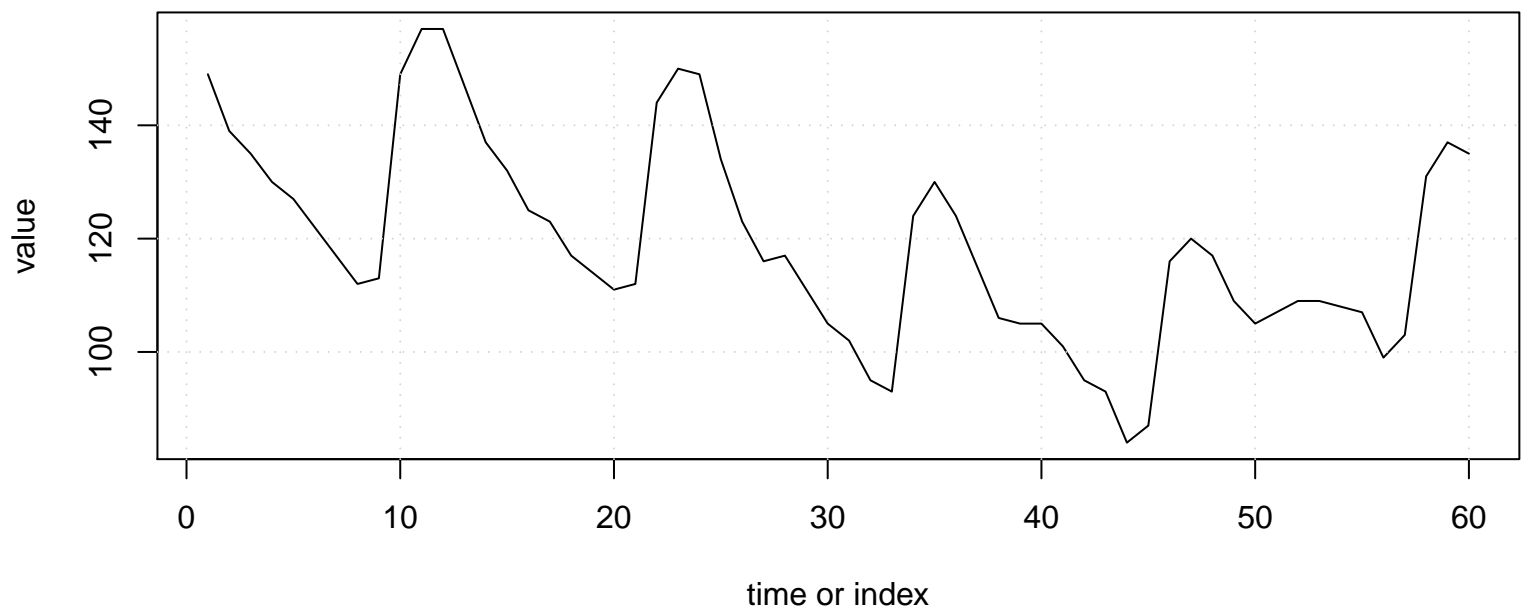
Run Sequence Plot of X[t]
