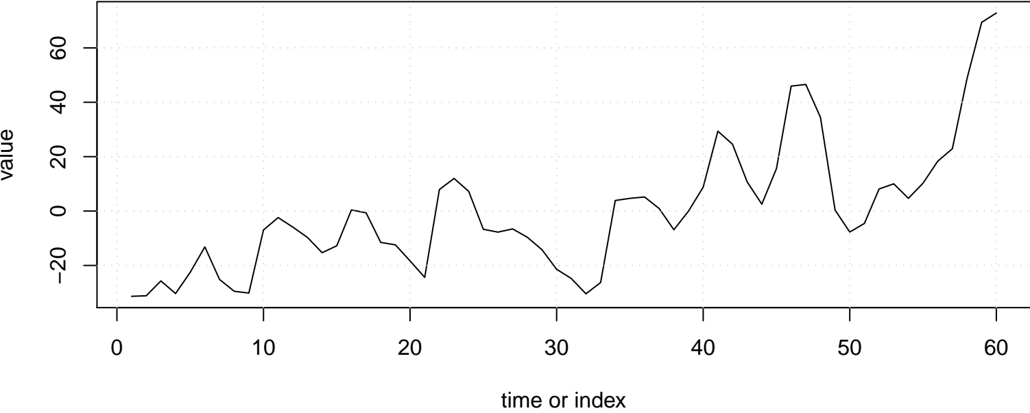
Run Sequence Plot of e[t]
