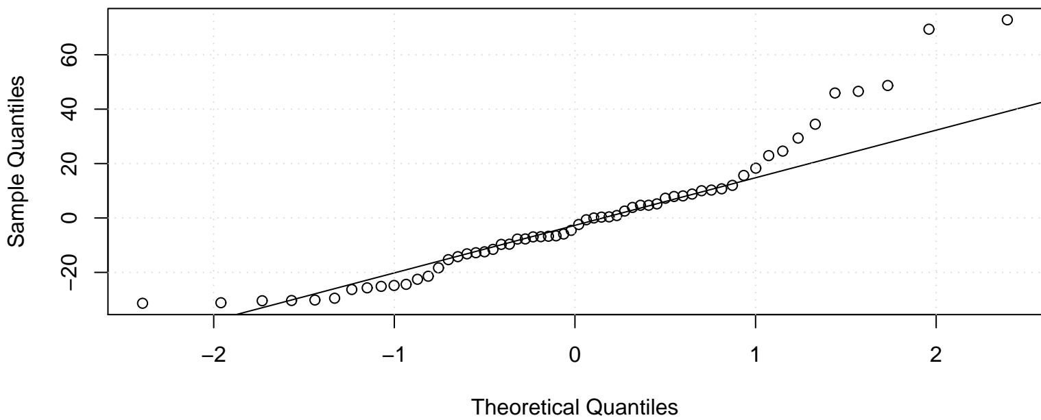
QQ plot of e[t]
