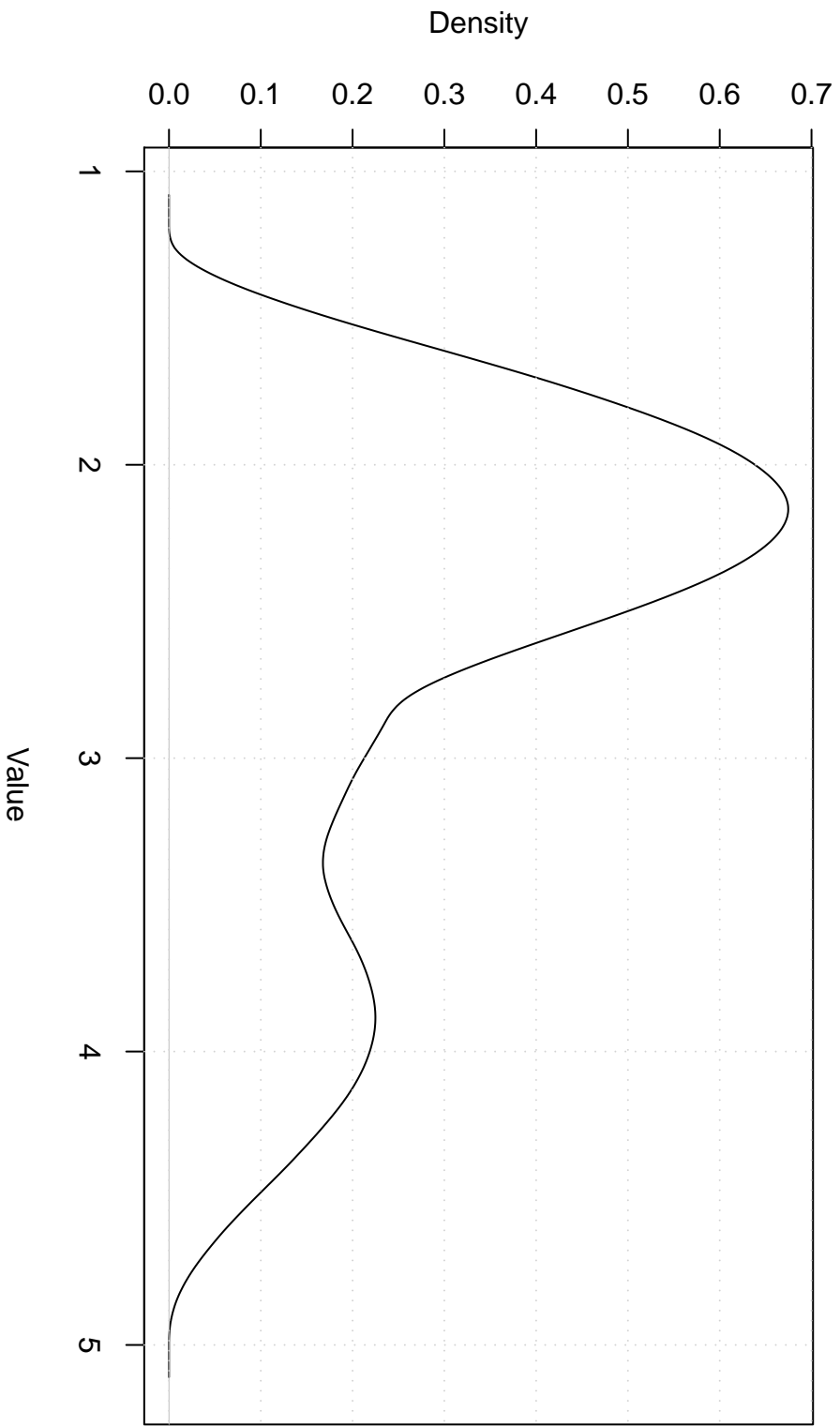
Biweight Kernel
