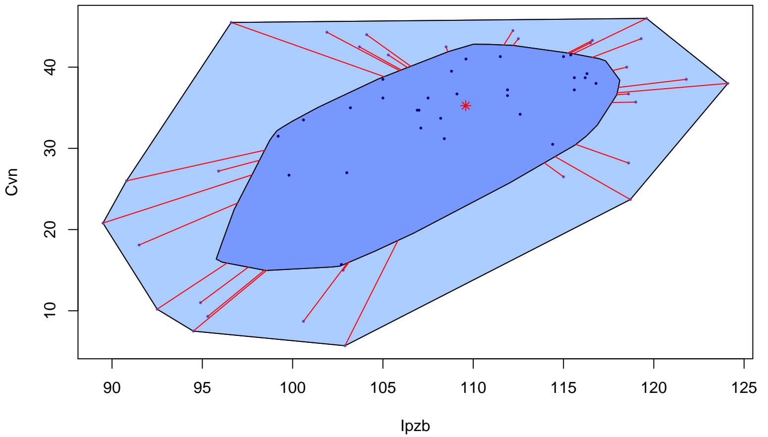
Bagplot
