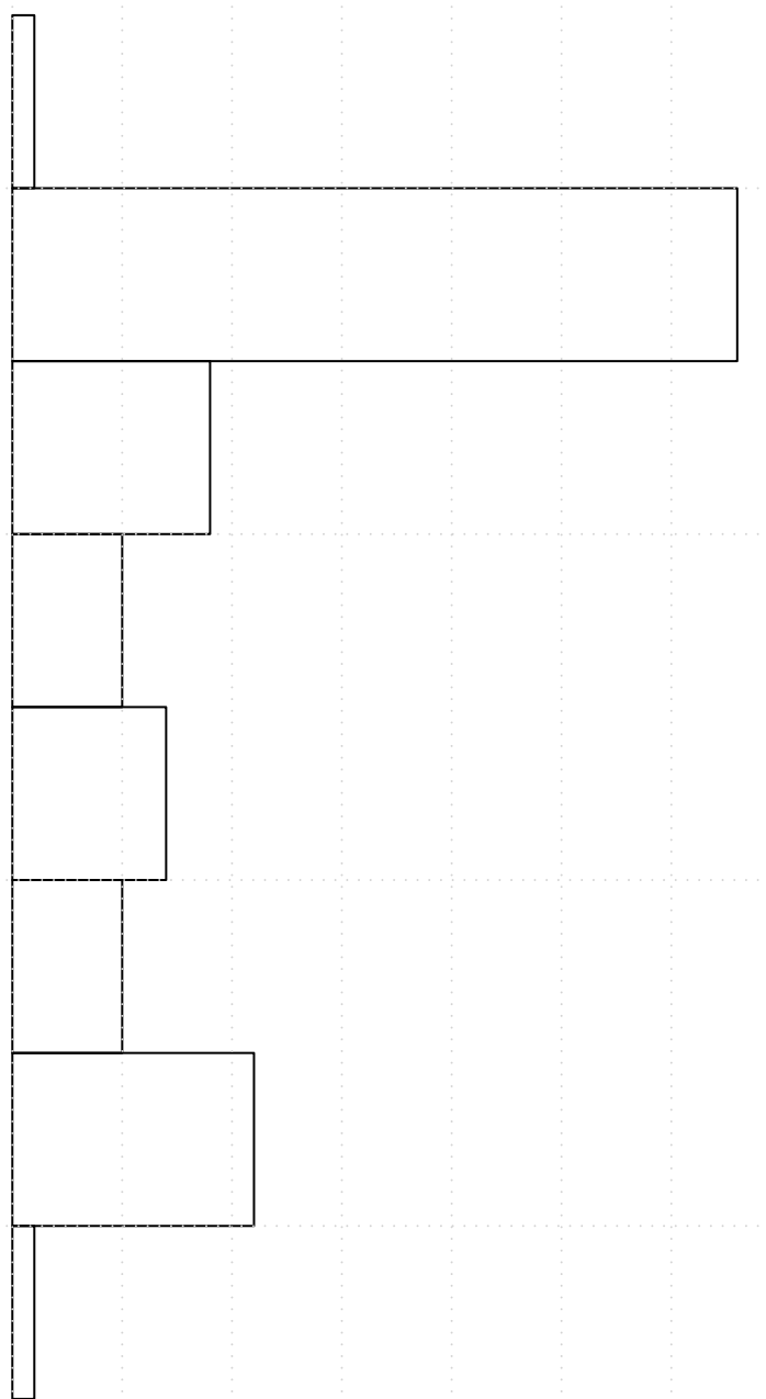
Histogram of x
