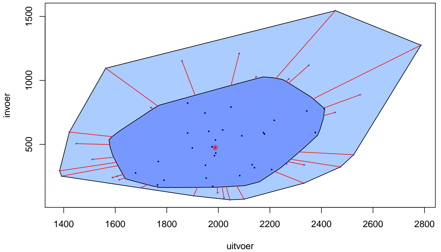
Bagplot
