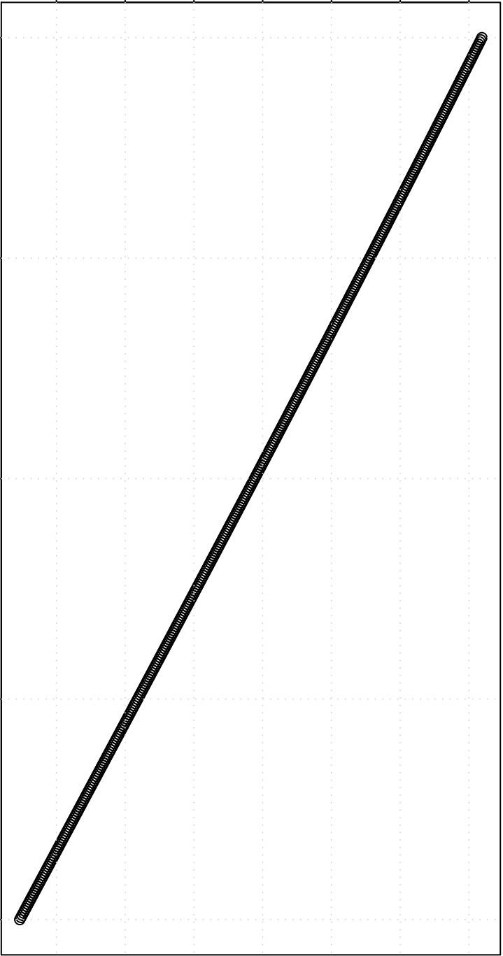
Box-Cox Linearity Plot
