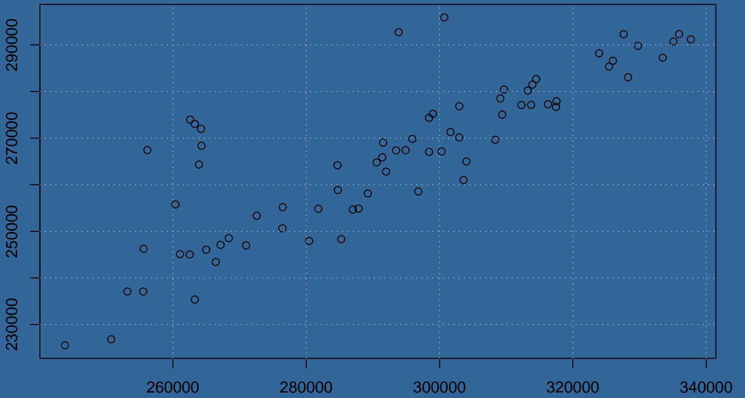
Scatterplot
