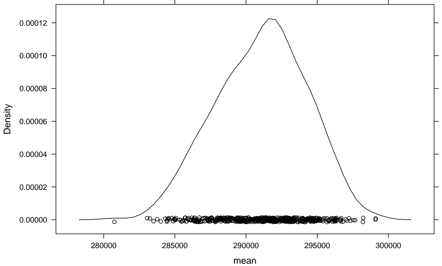
Density Plot
