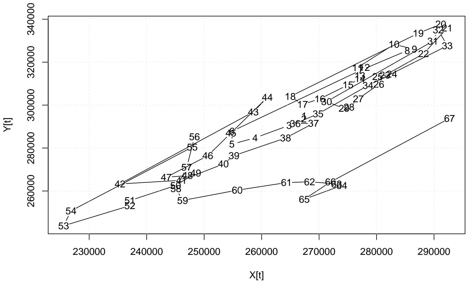
Scatter Plot
