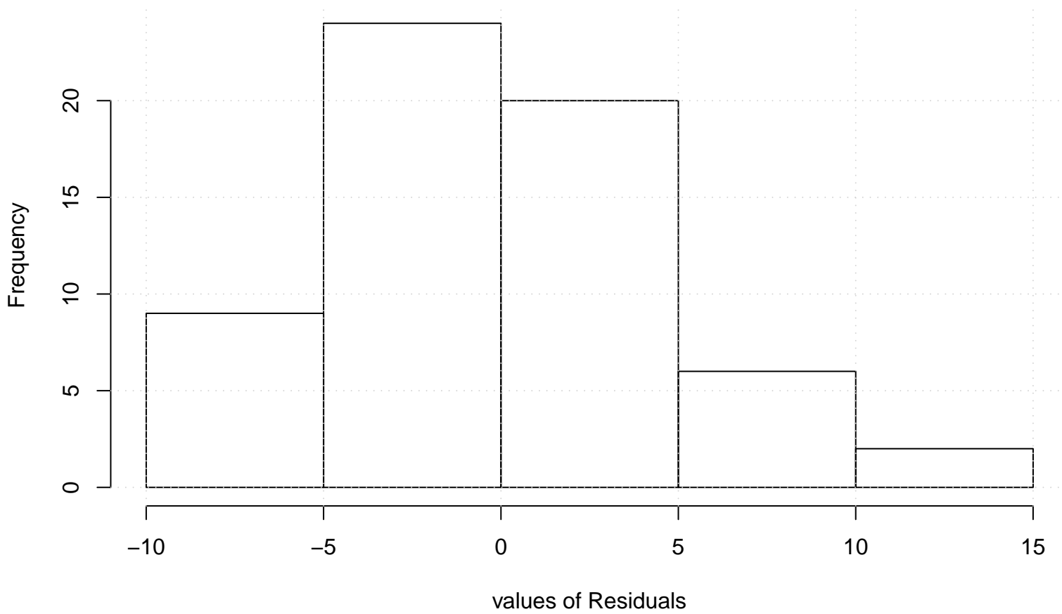
Residual Histogram
