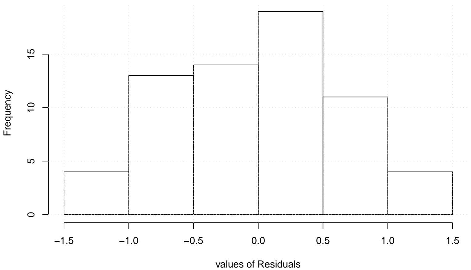
Residual Histogram
