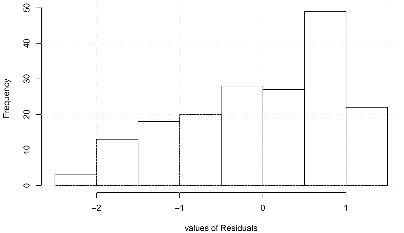
Residual Histogram
