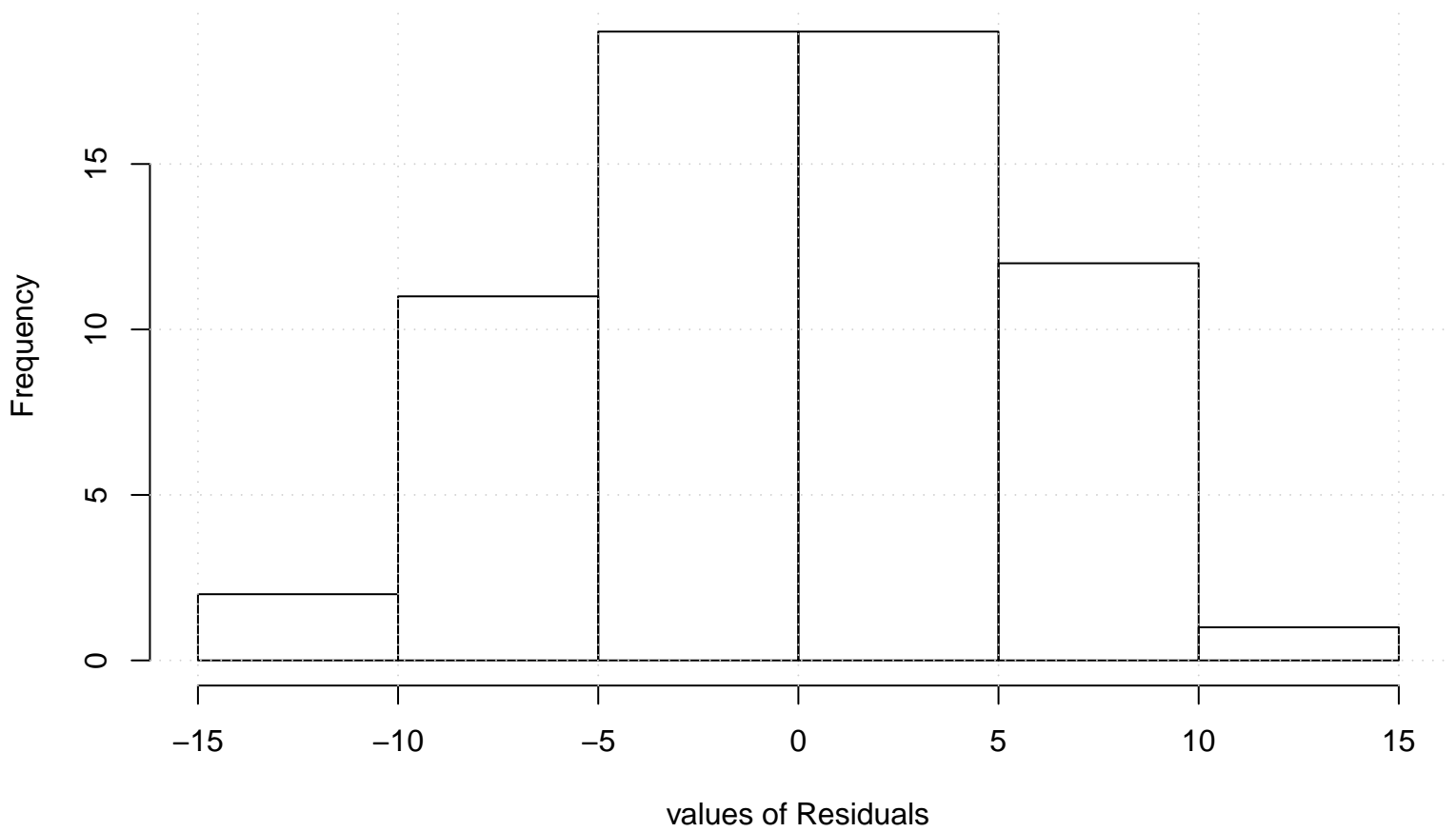
Residual Histogram
