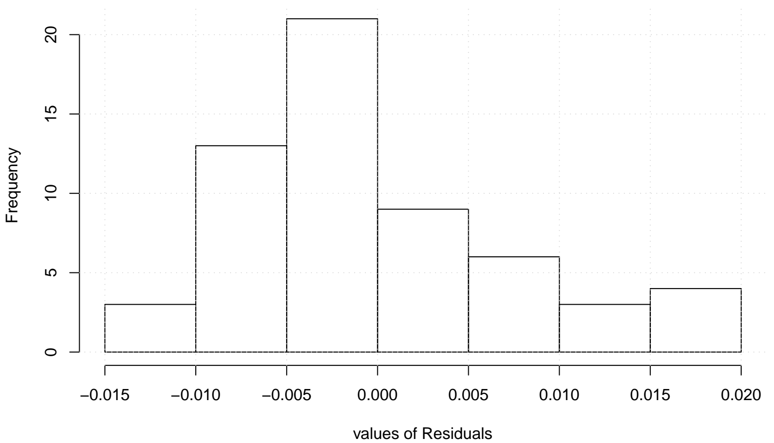
Residual Histogram
