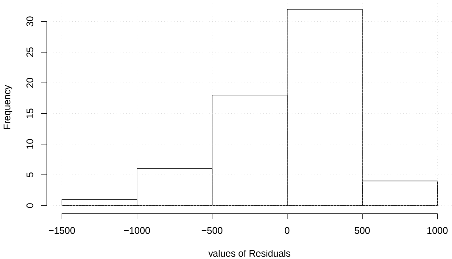
Residual Histogram
