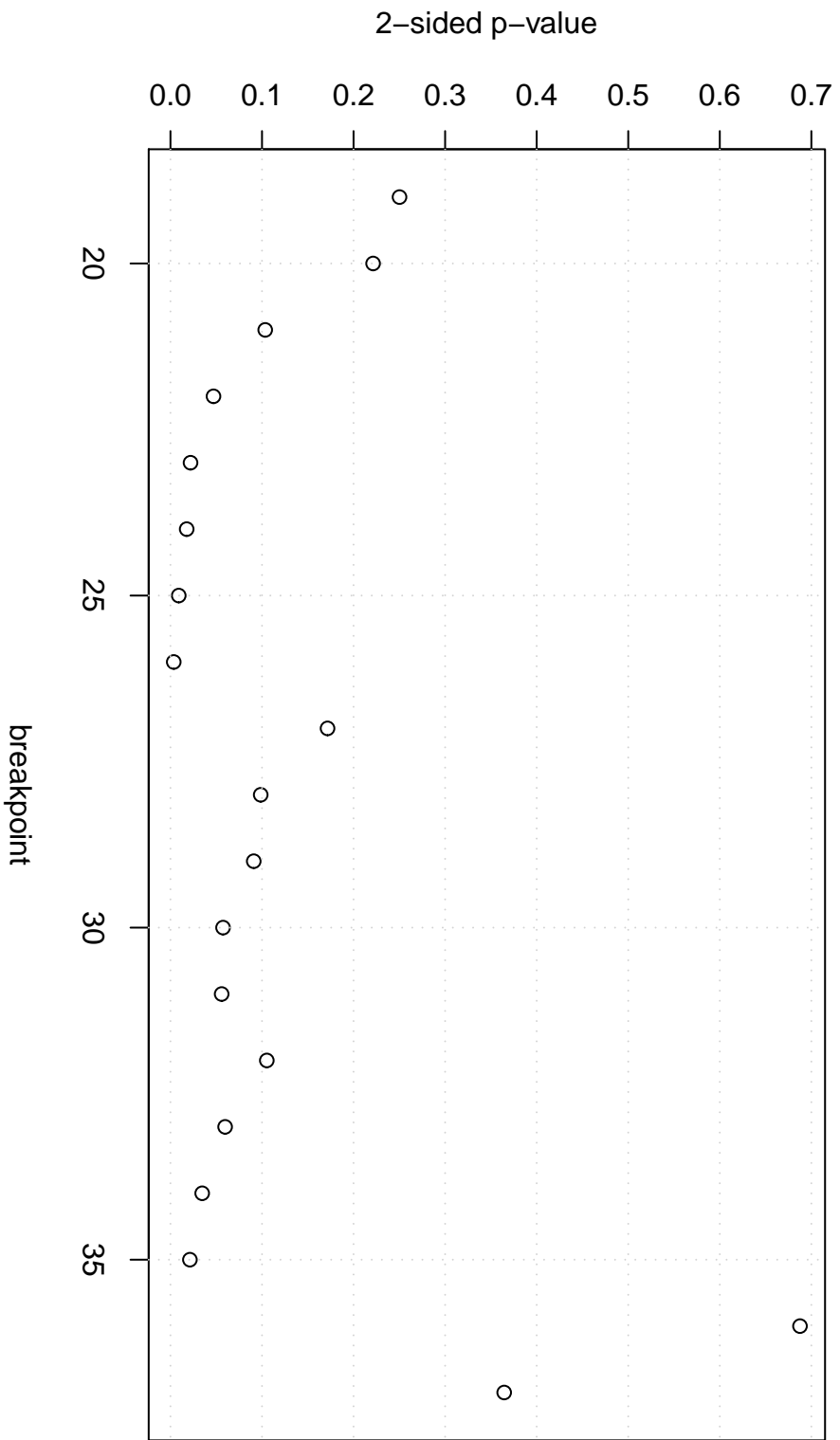
Goldfeld-Quandt test
