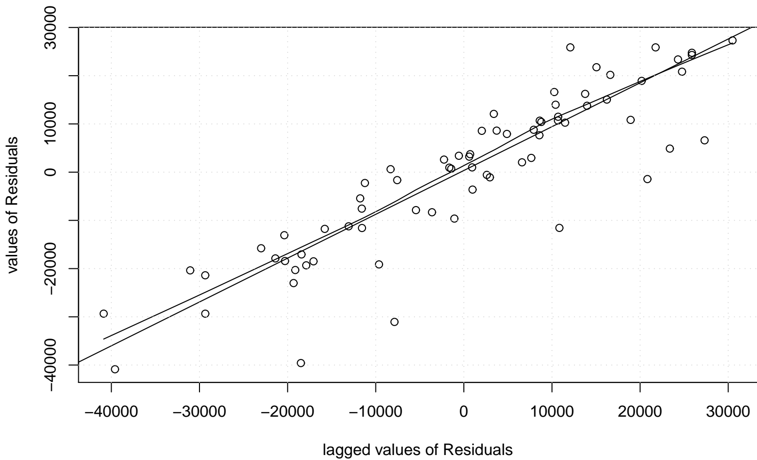
Residual Lag plot, lowess, and regression line
