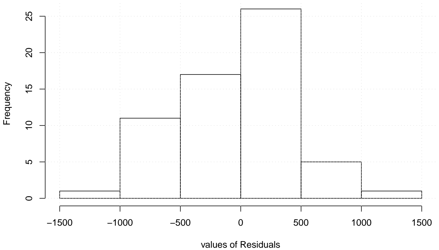
Residual Histogram
