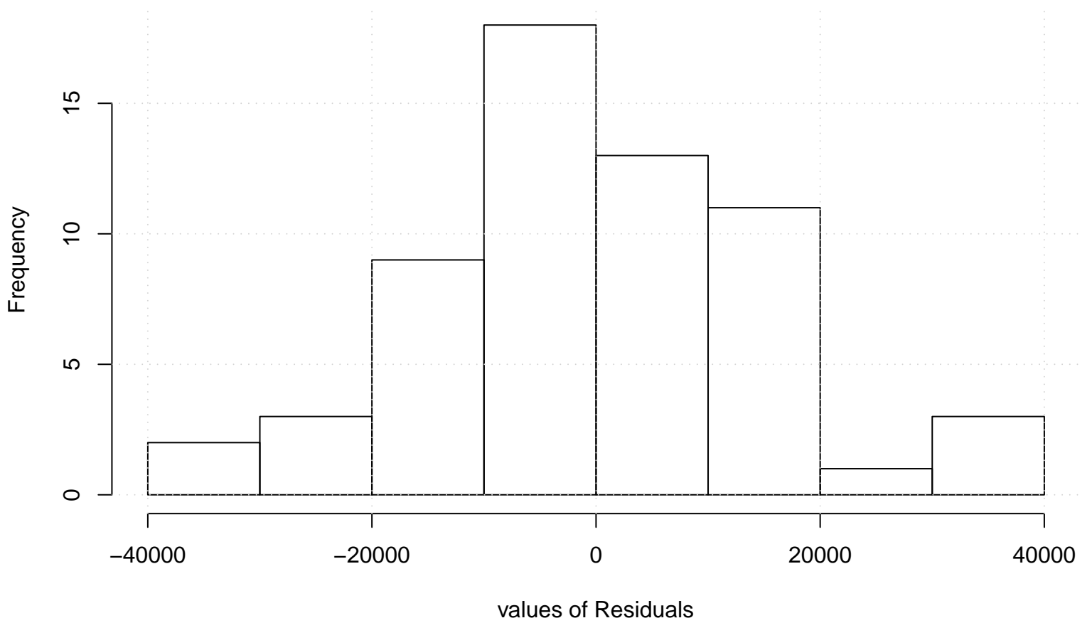
Residual Histogram
