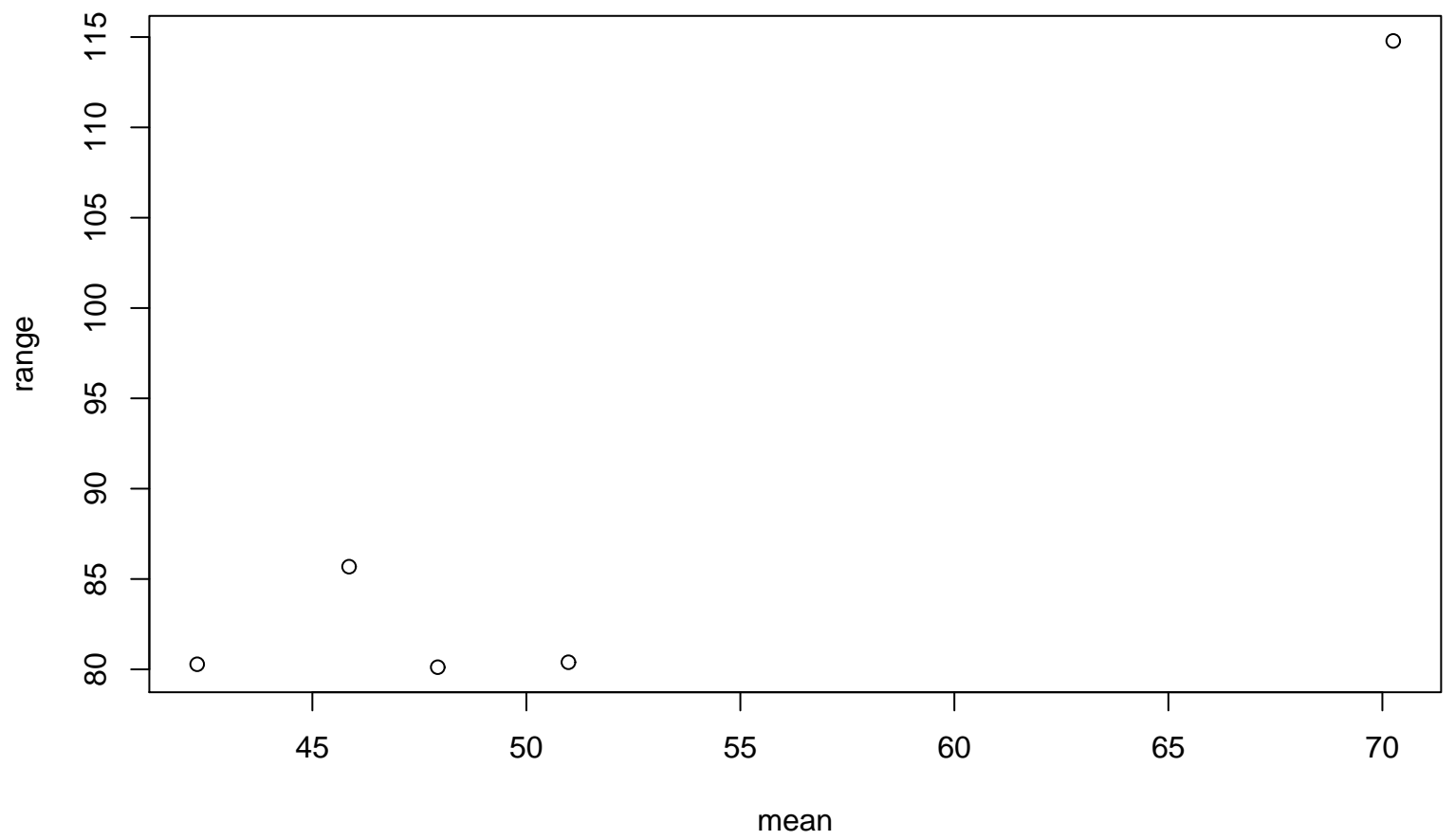
Range-Mean Plot
