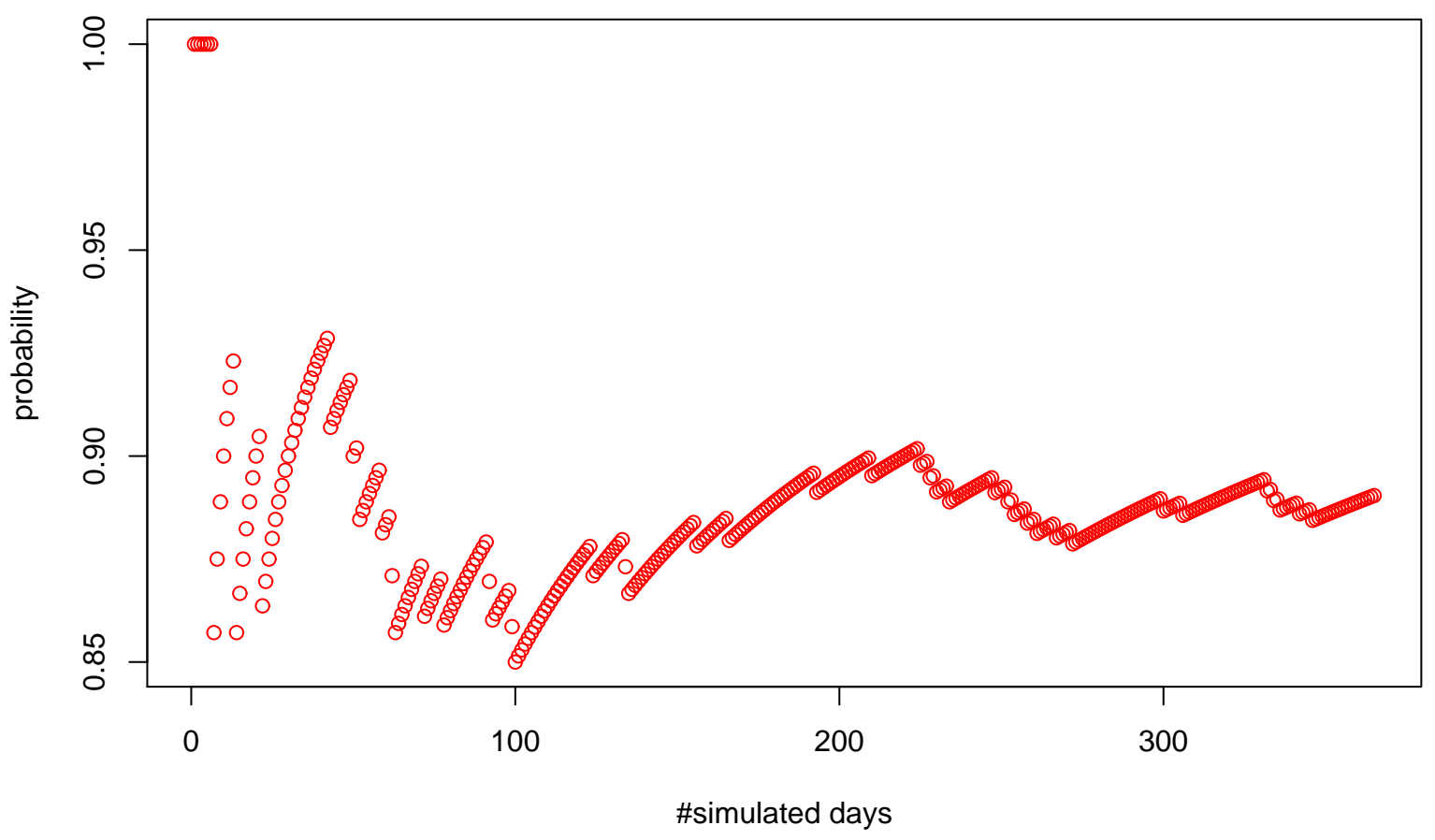
Probability of less than 60 % of male births in Large Hospital
