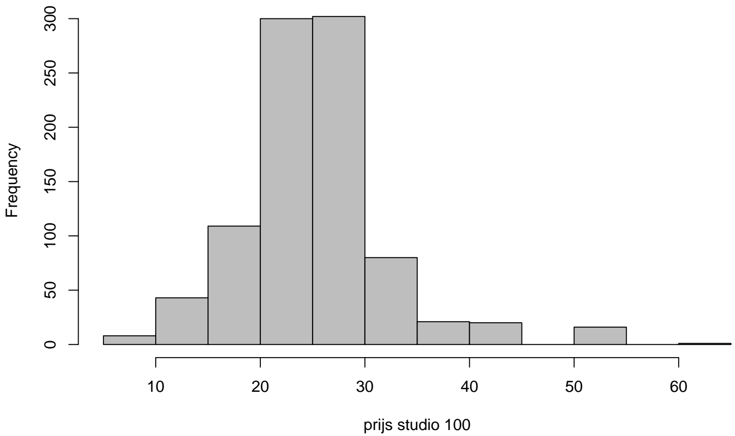
studio 100 histogram
