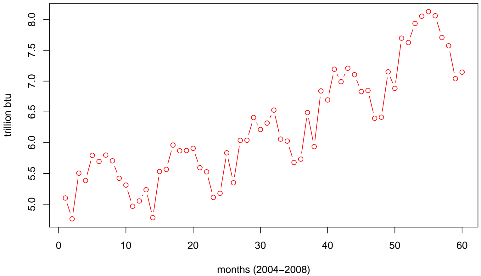
consumed solar energy in the US
