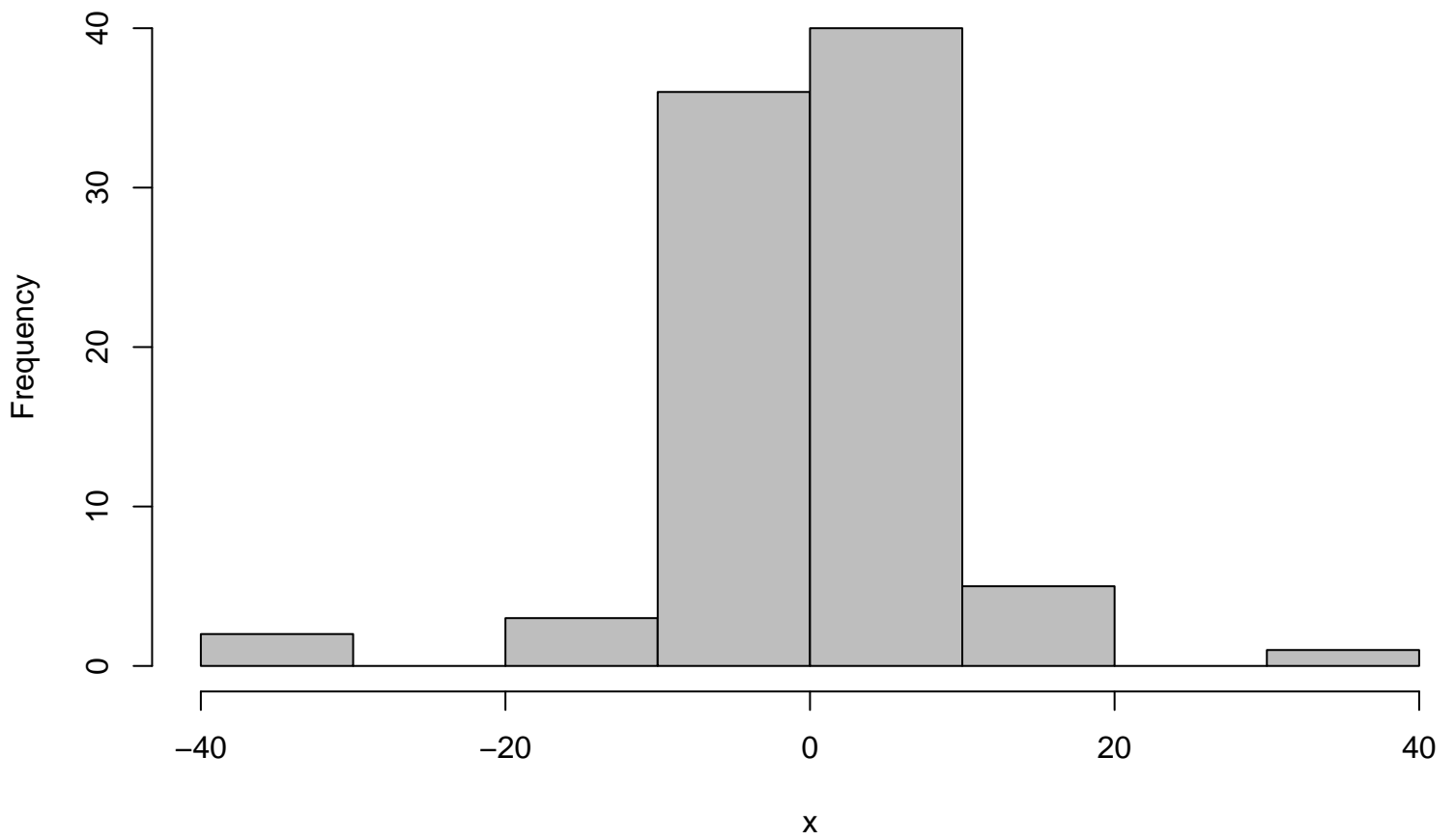
Histogram X(t)/Y(t)
