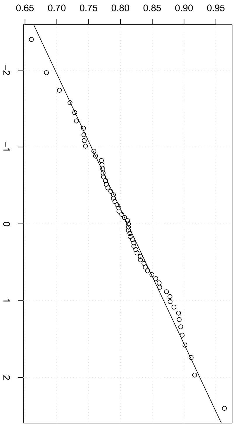
Sample Quantiles
