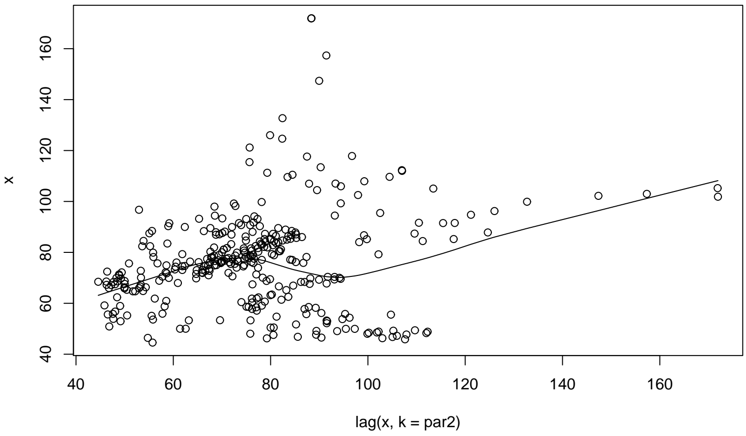
Lag plot (k=24), and lowess
