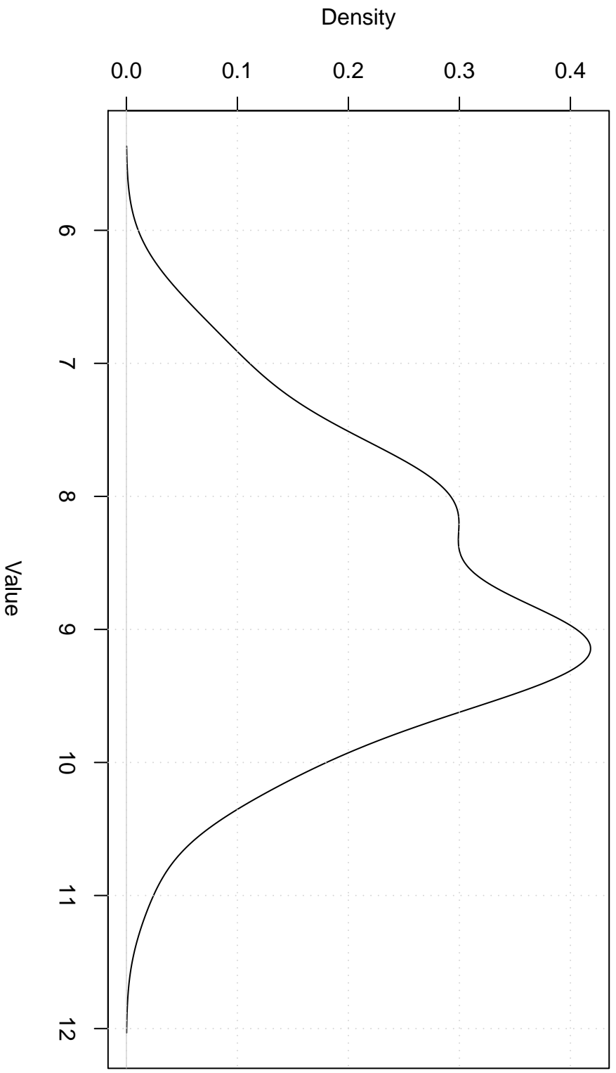
Gaussian Kernel
