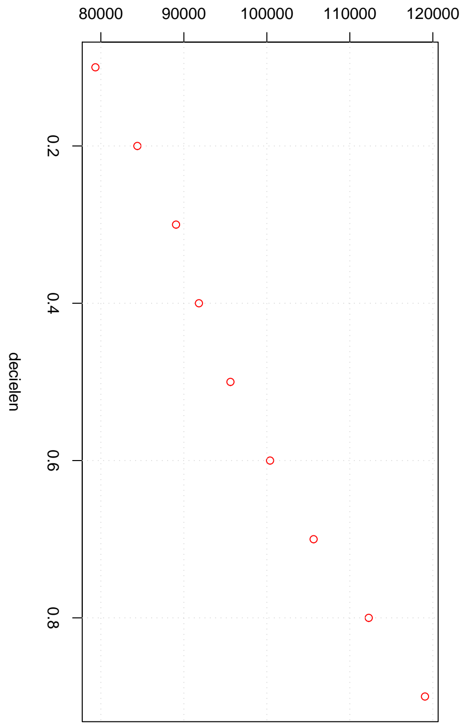
Harrell-Davis Quantiles
