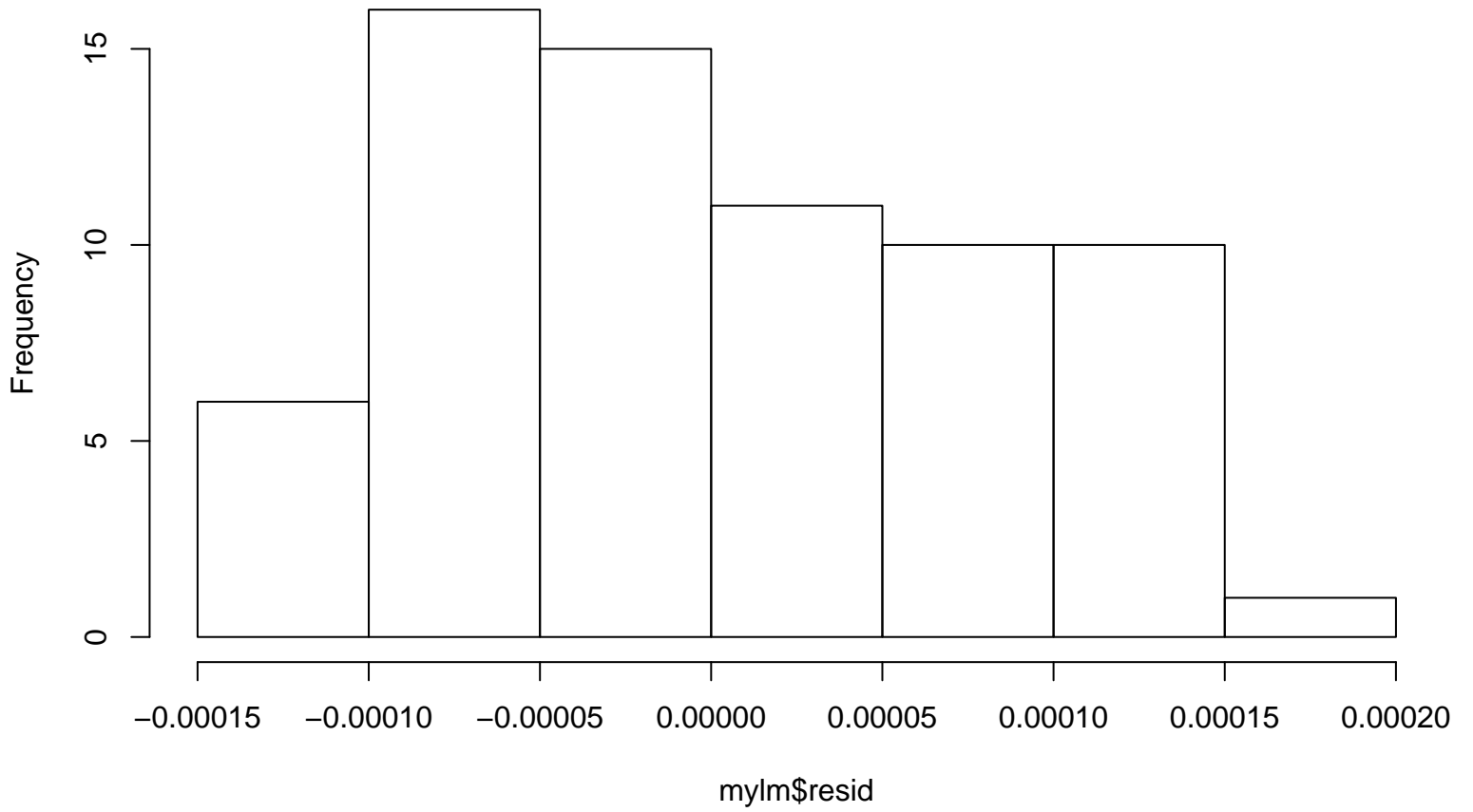
Histogram of e[t]
