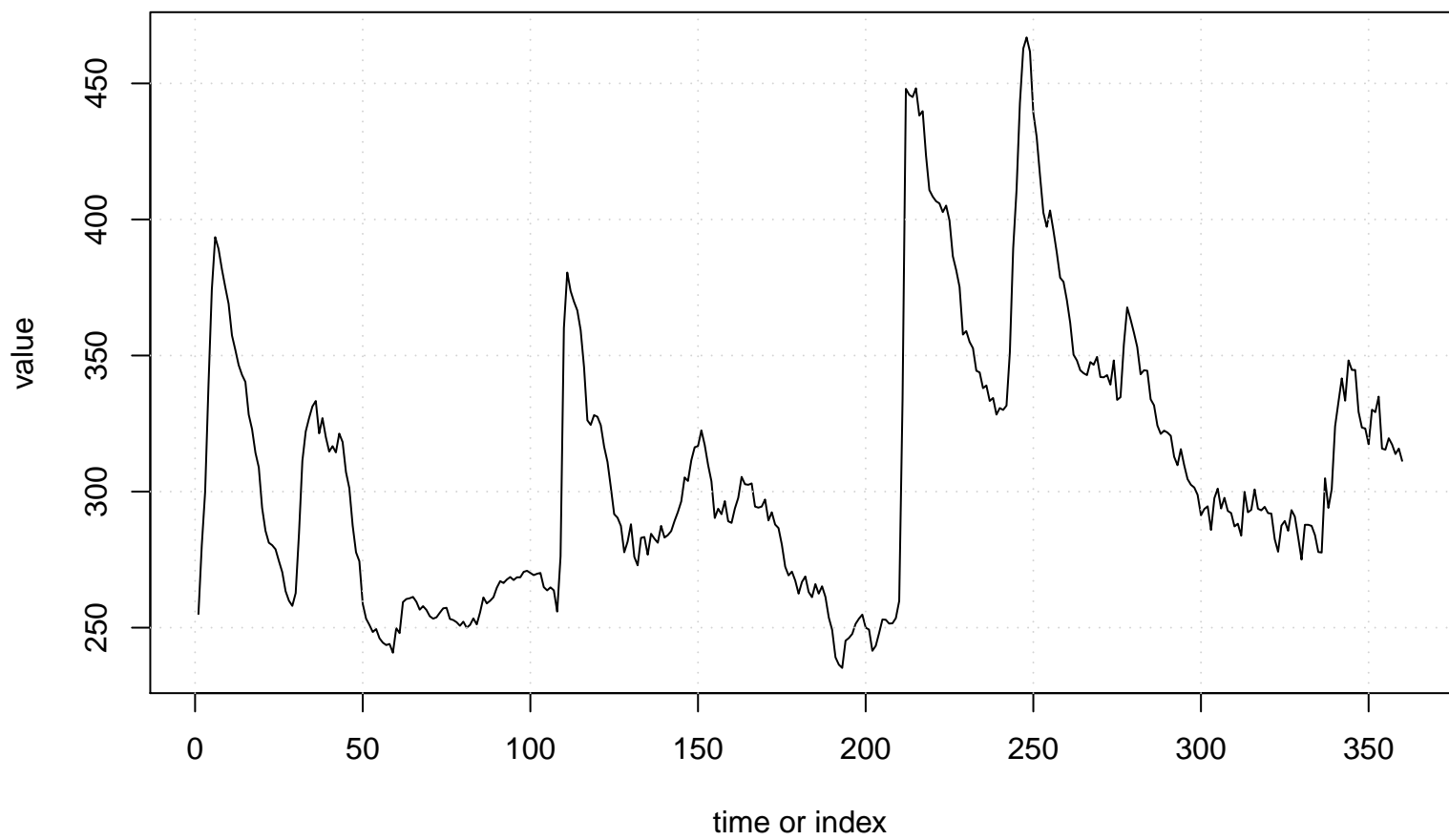
Run Sequence Plot of Y[t]
