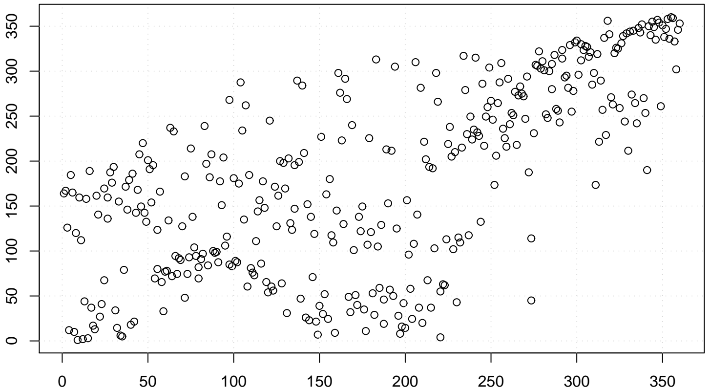
Scatterplot of Ranks
