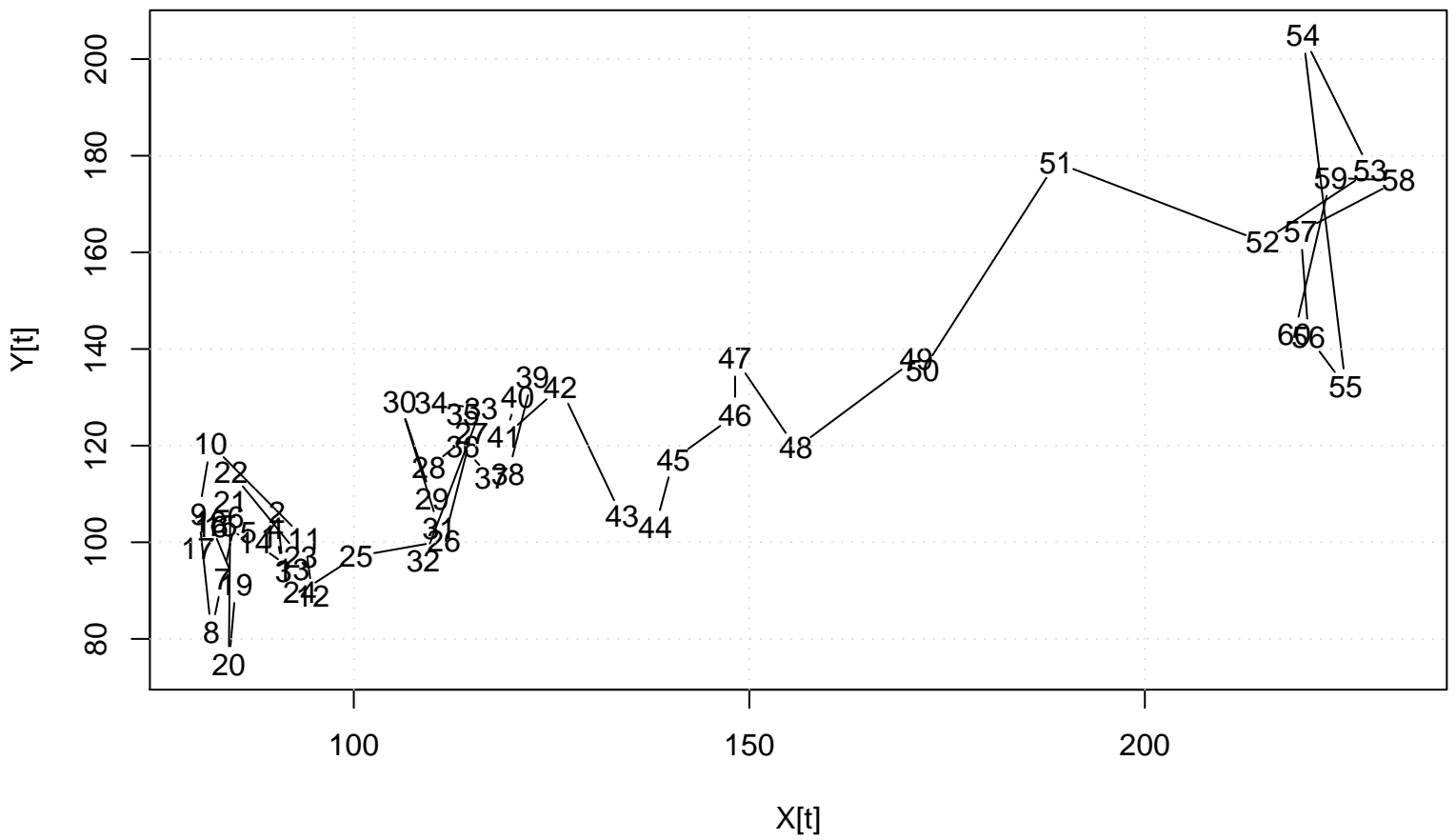
Scatter Plot
