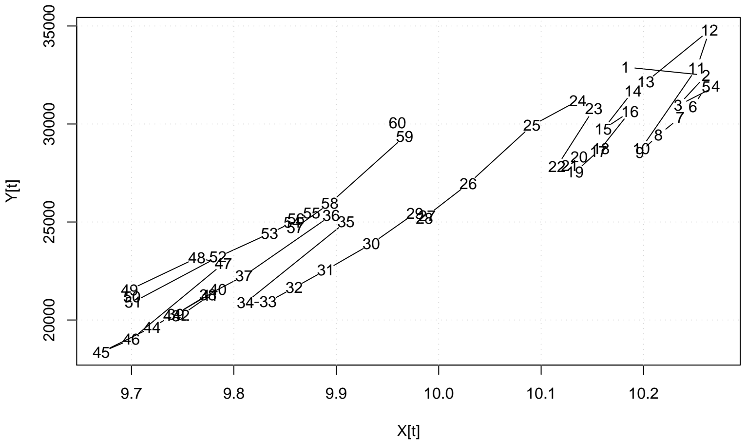
Scatter Plot
