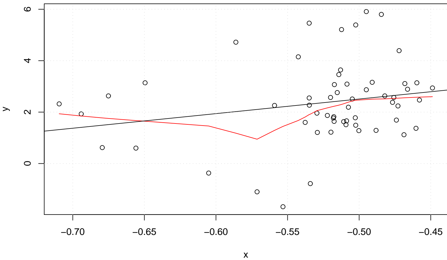
Scatterplot, lowess, and regression line
