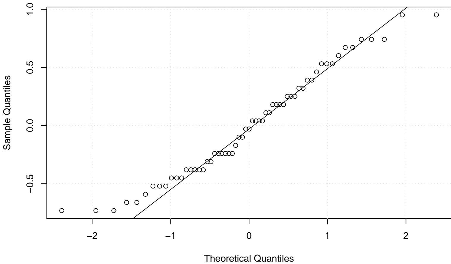
QQ plot of e[t]
