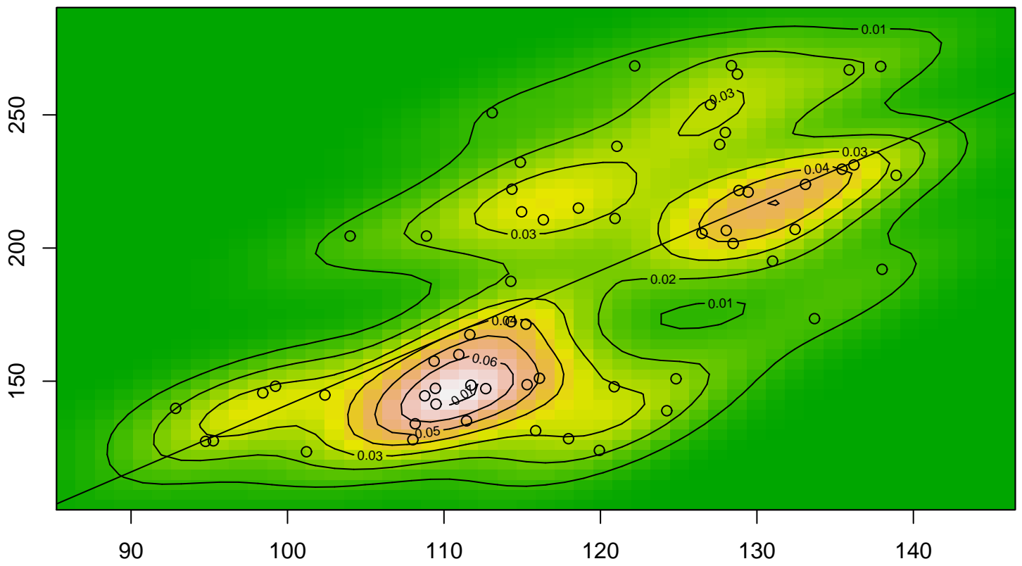
Bivariate Kernel Density Plot (y,z)
