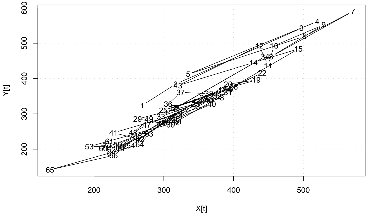
Scatter Plot
