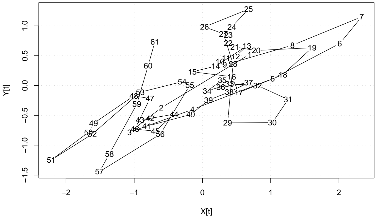
Scatter Plot
