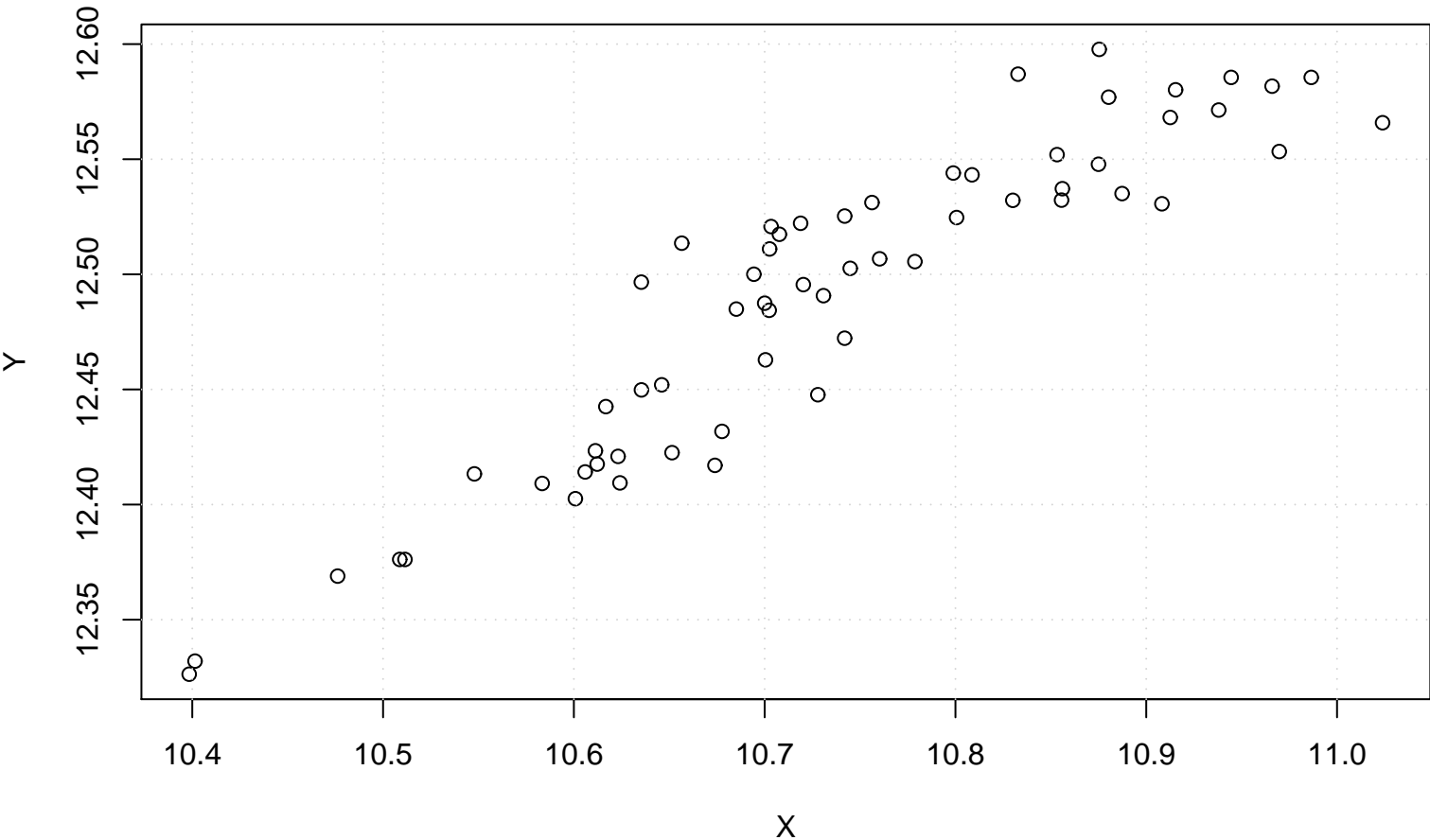
Scatterplot
