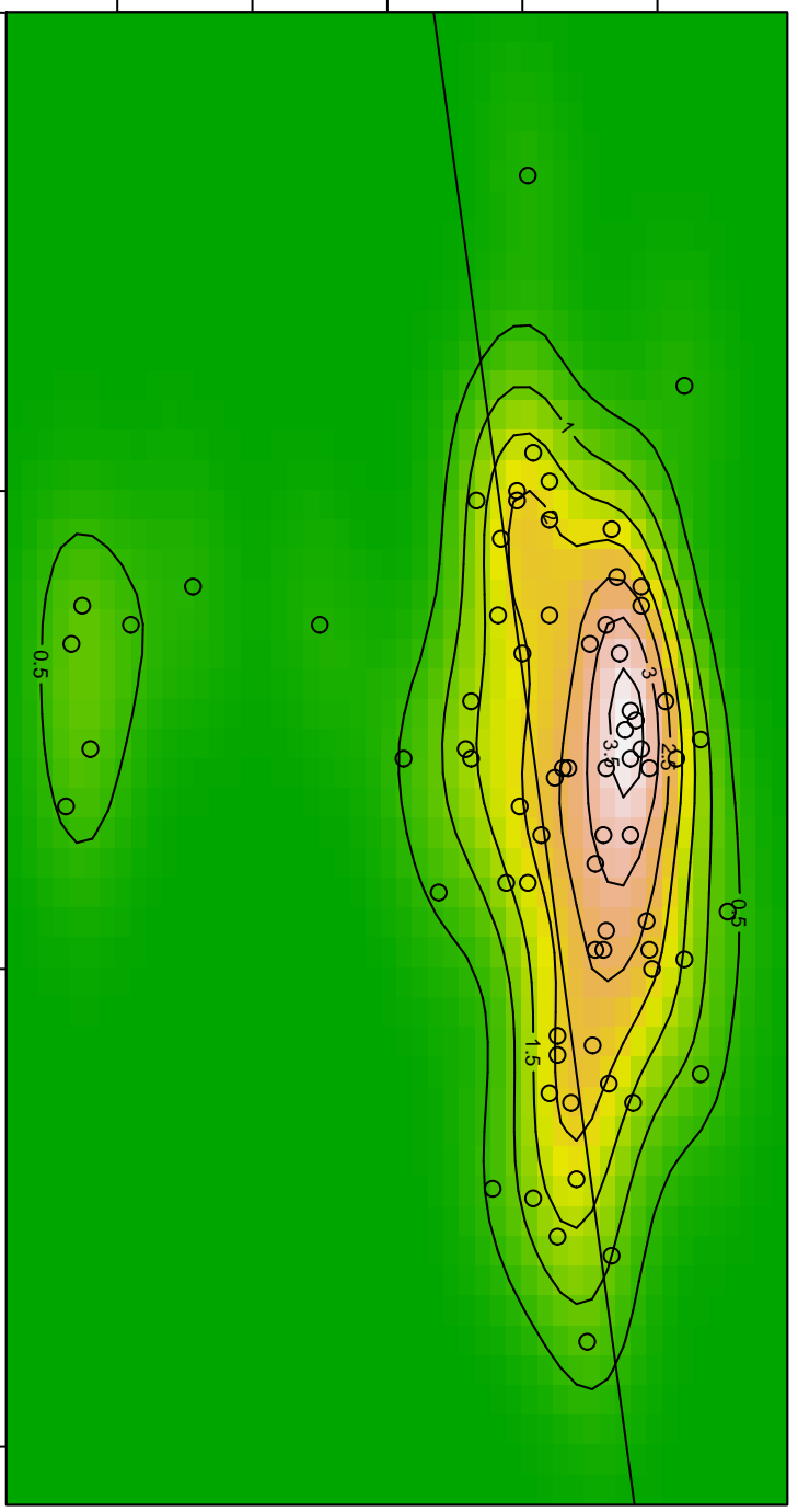
Bivariate Kernel Density Plot (x,z)
