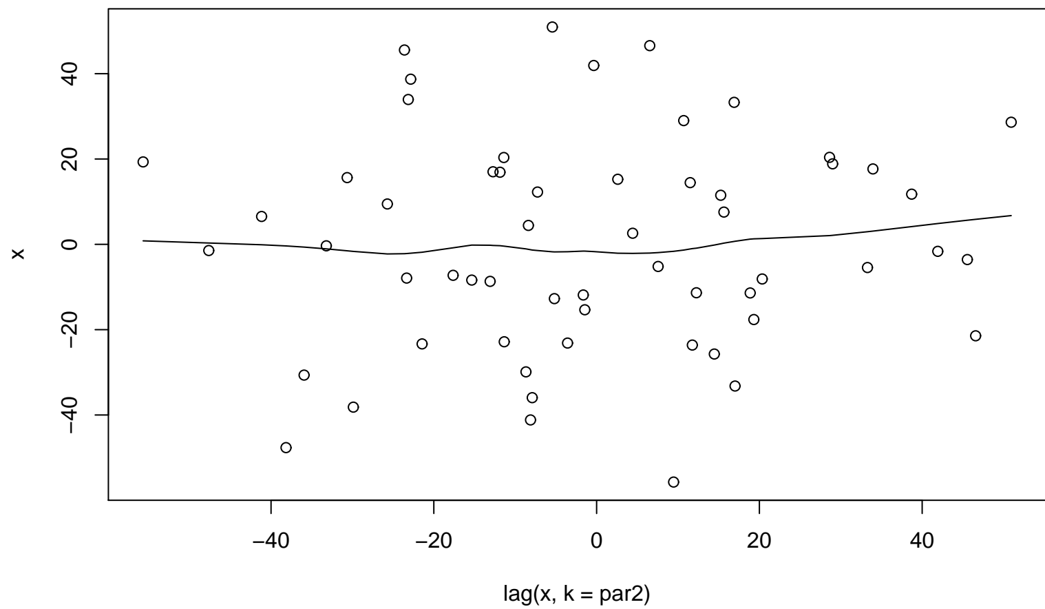
Lag plot (k=2), and lowess
