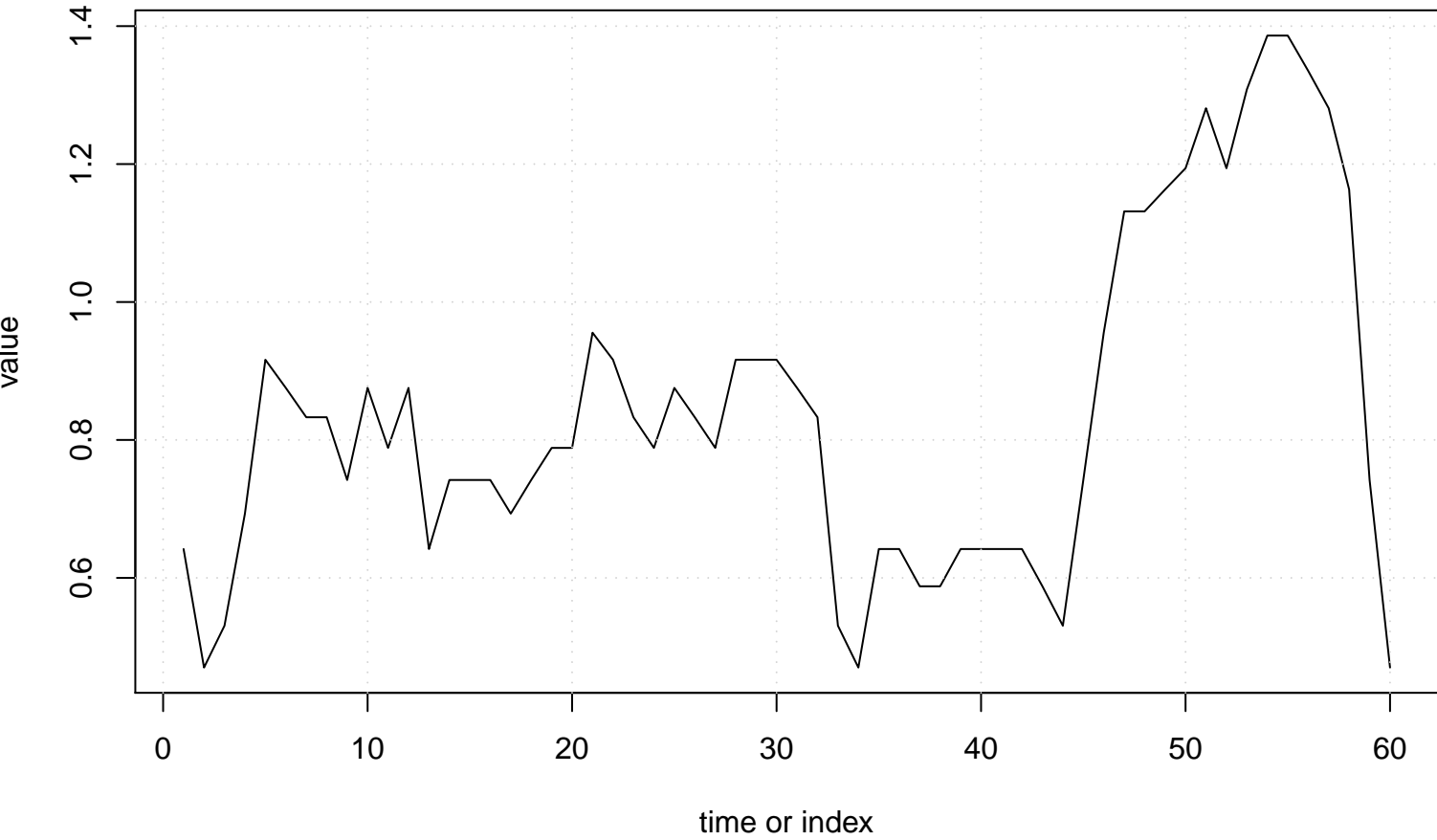
Run Sequence Plot of Y[t]
