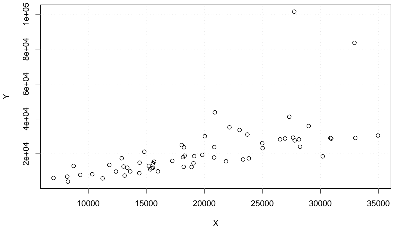
Scatterplot
