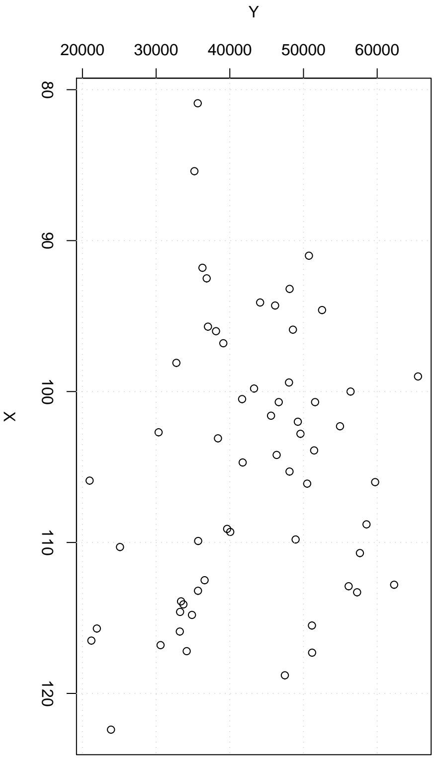
Scatterplot
