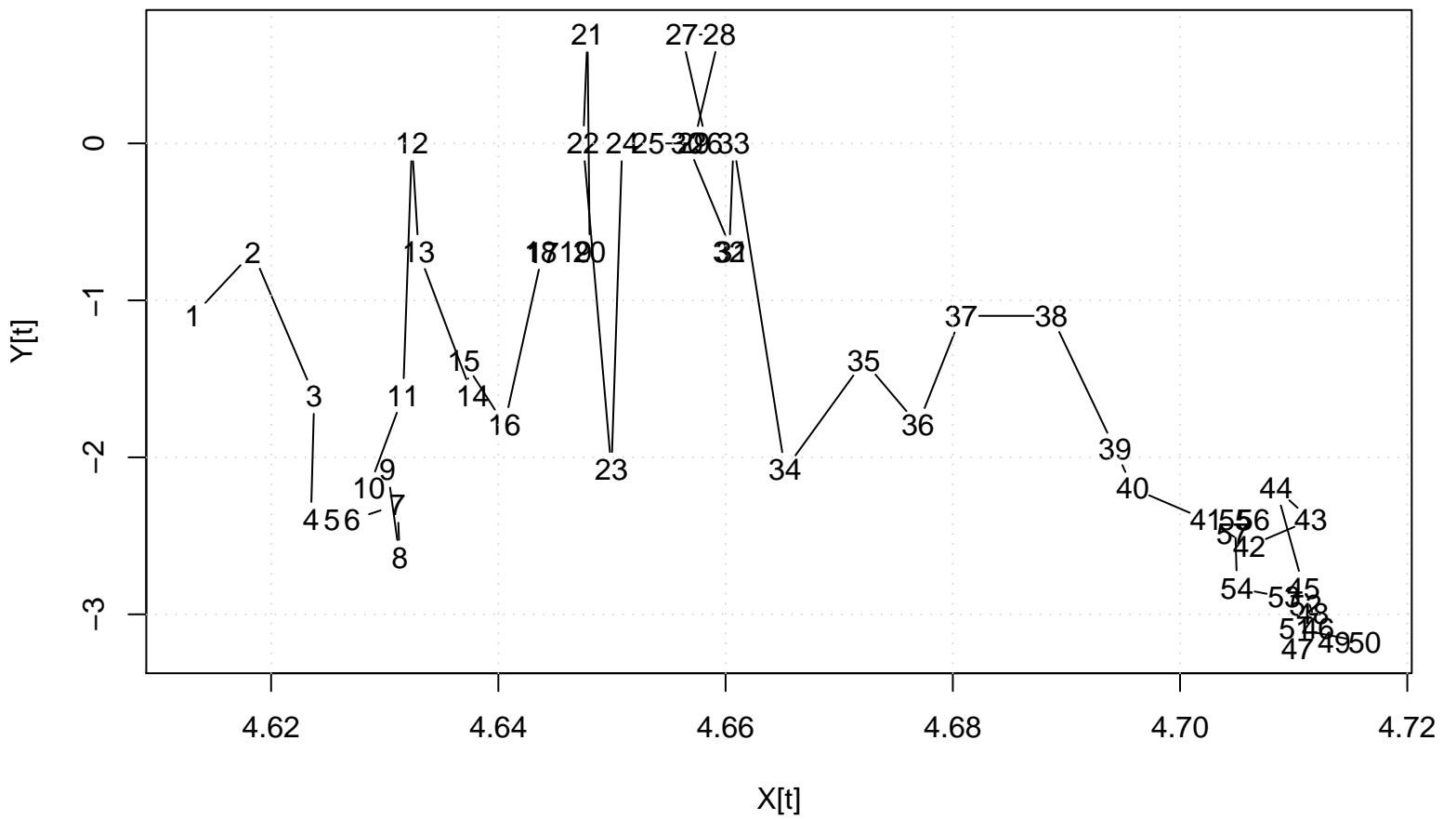
Scatter Plot
