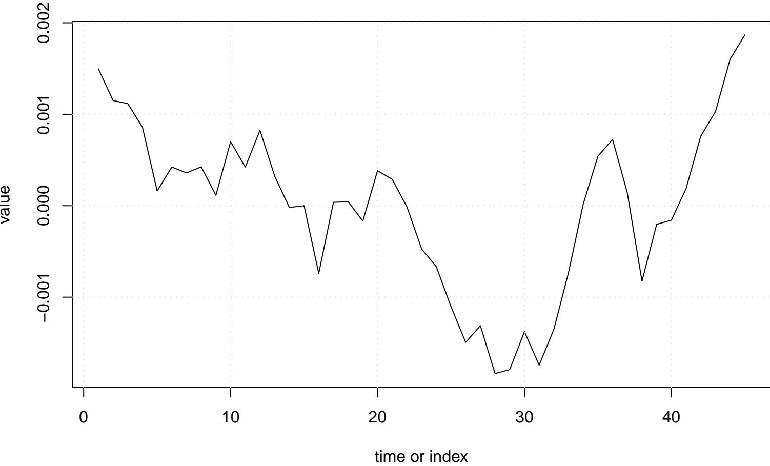
Run Sequence Plot of e[t]
